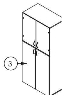
800x470x1780 3M/2M sklo (glass) FT-D
