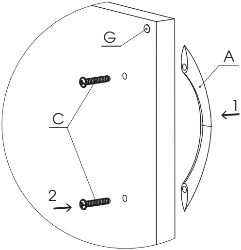
DETAIL 1
