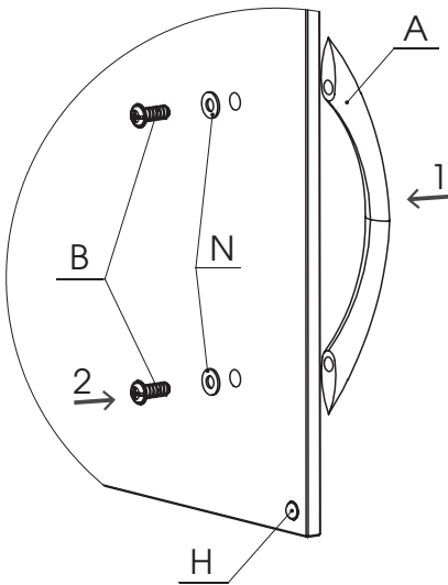
DETAIL 2
