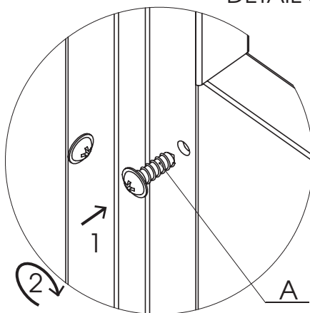
DETAIL 3
